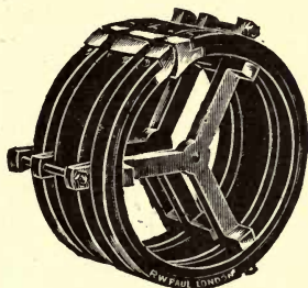
Fig. 69.—Astatically Arranged Permanent Magnets
